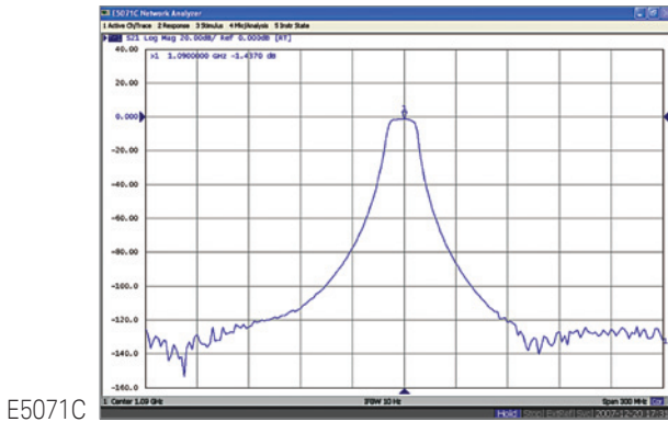
E5071C 动态范围对比: IFBW = 10 Hz
