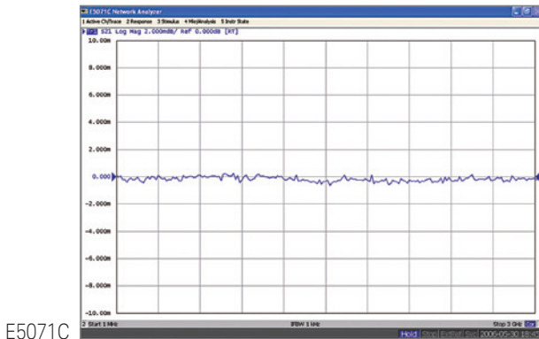
E5071C 轨迹噪声对比: IFBW = 1 kHz
